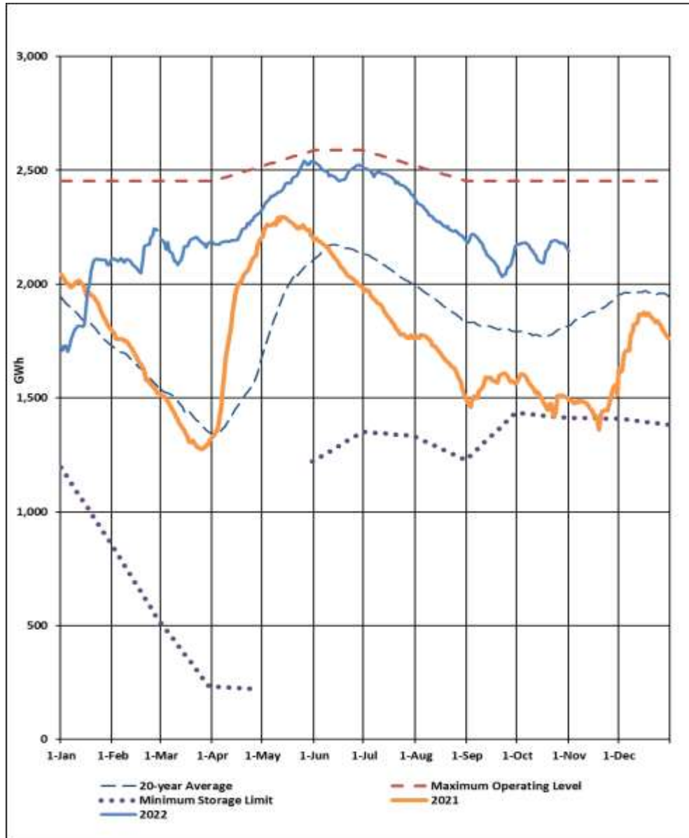
Chart 1: Total System Energy Storage for October 31, 2022
